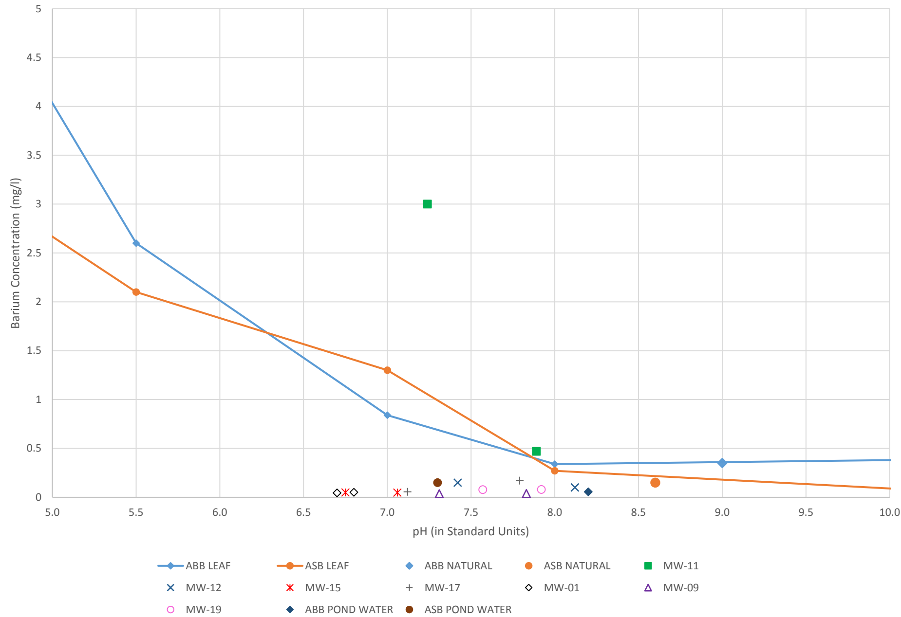
Figure 3a. Barium Concentration vs. pH Value - Powerton Station (May/August 2018 Data)
