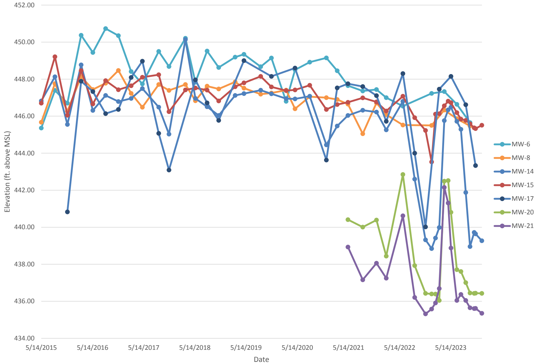
Figure 2-3. Powerton Silt/Clay Wells Hydrograph
