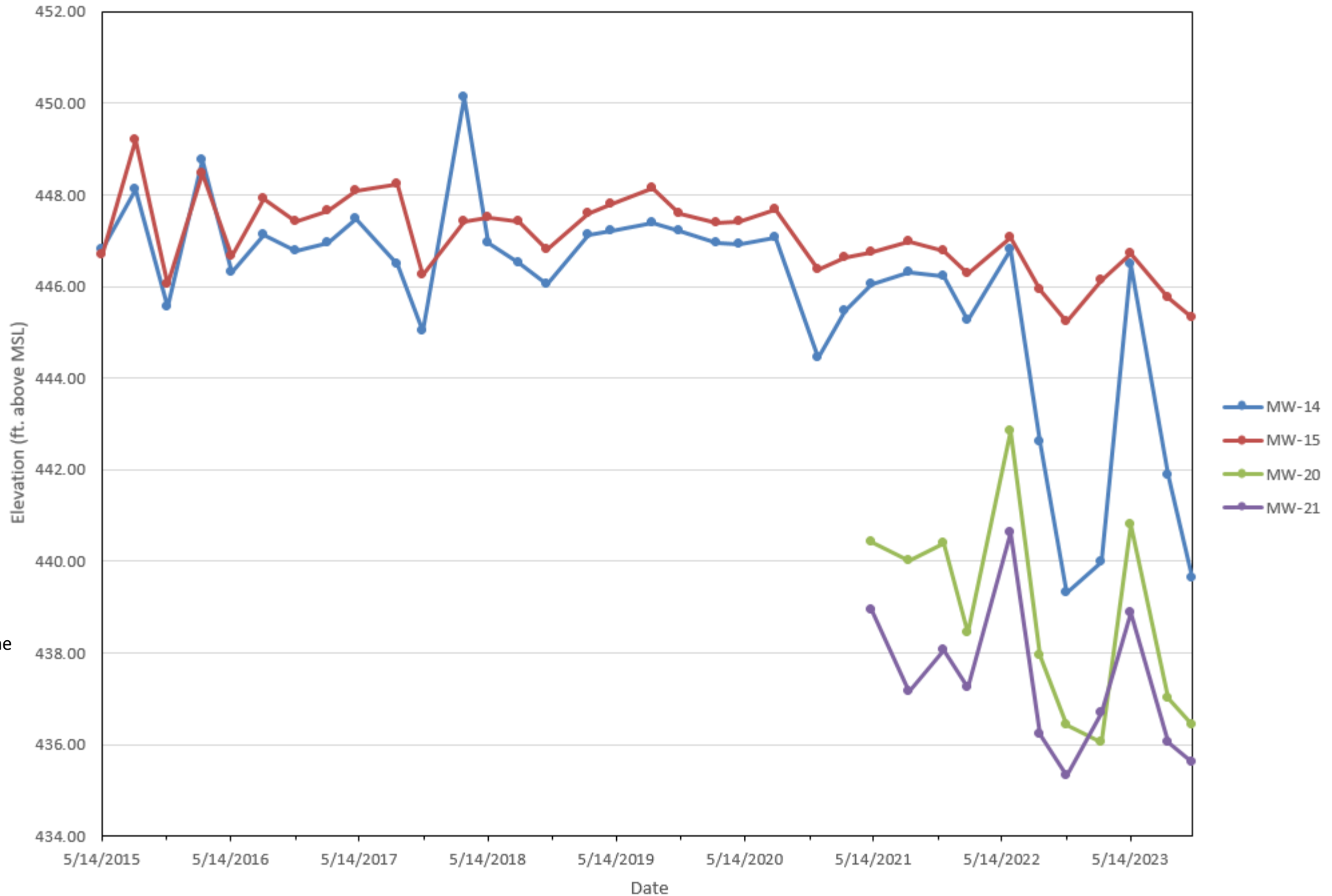
Figure 2-2 Powerton Silt/Clay Wells Hydrograph
